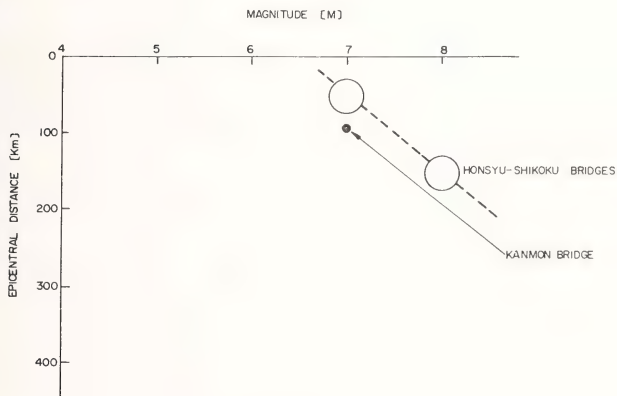
Fig. I-3 GROUND MOTIONS USED FOR SEISMIC ANALYSES OF SUSPENSION BRIDGES CONSTRUCTED OR PLANNED TO CONSTRUCT
